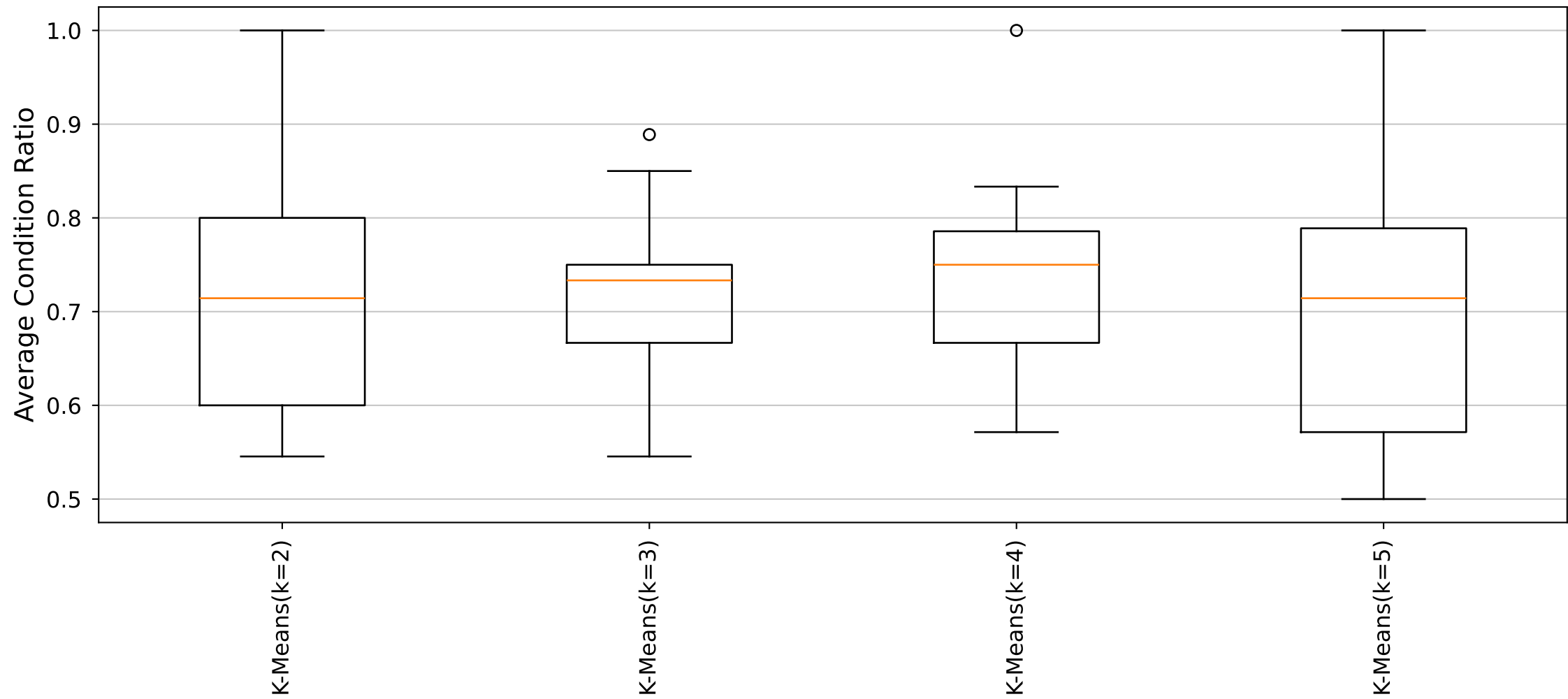
YARA Rules Average Condition Ratio Distribution (Cluster45_Size5 dataset)
